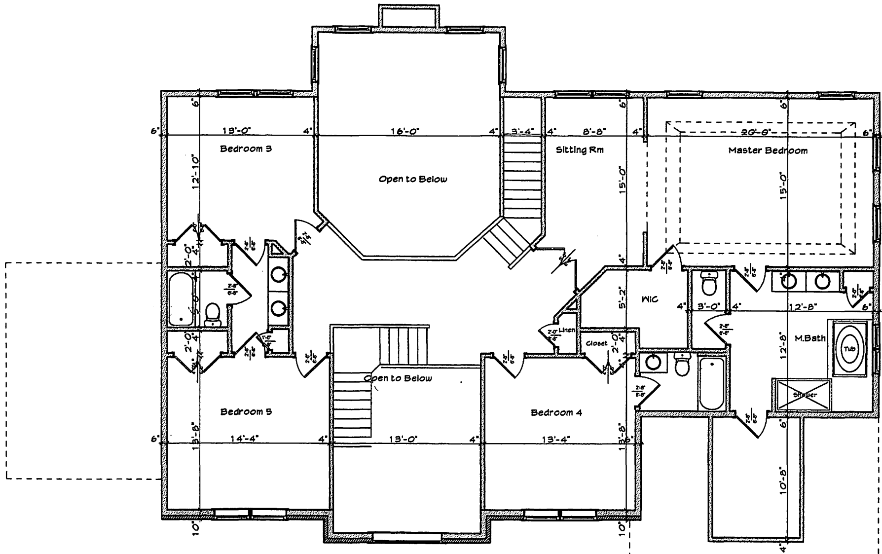
Second Floor Plan 1,778.52 sq ft
